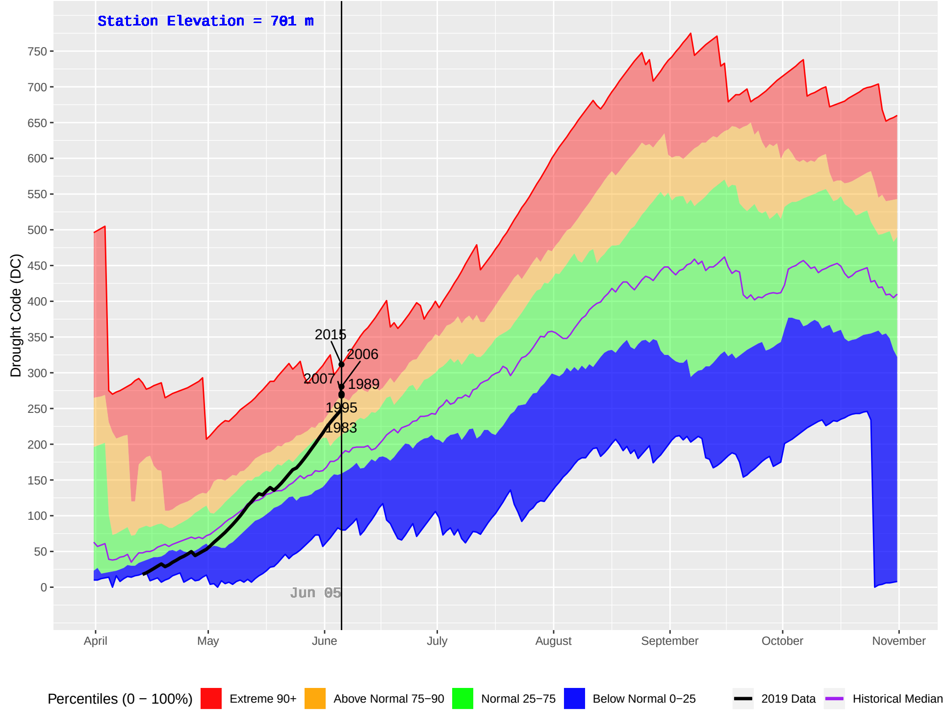
HORSEFLY (230) : Historical (1971–2018) and Current (2019) Daily Drought Code (DC)
