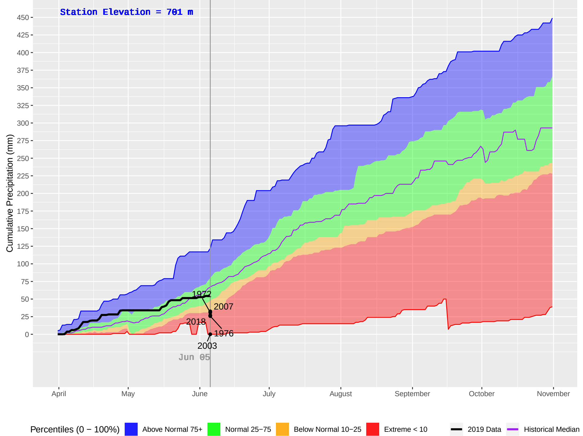
HORSEFLY (230) : Historical (1971–2018), Current (2019) Daily Cumulative Precipitation
