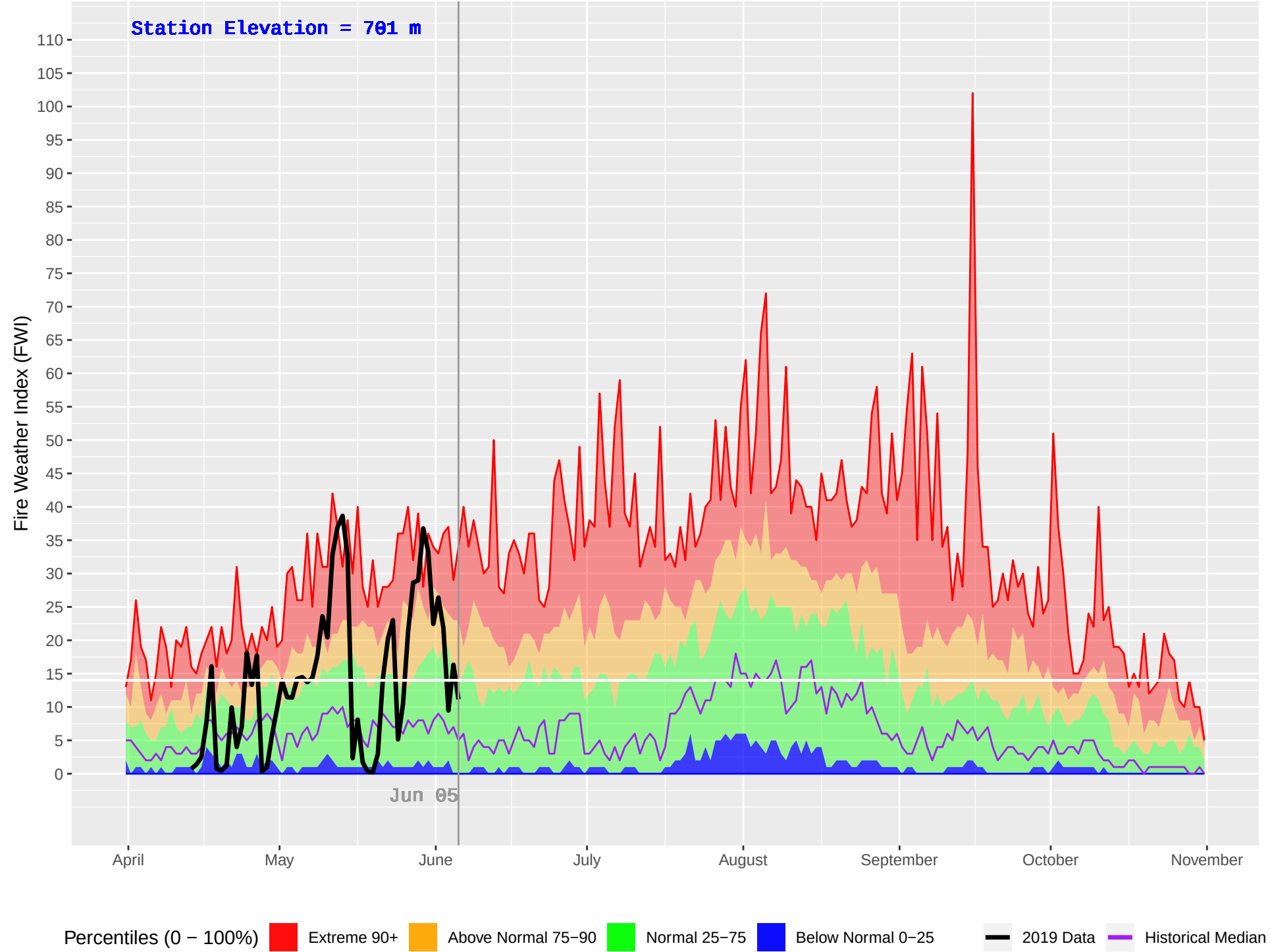
HORSEFLY (230) : Historical (1971–2018) and Current (2019) Daily Fire Weather Index (FWI)
