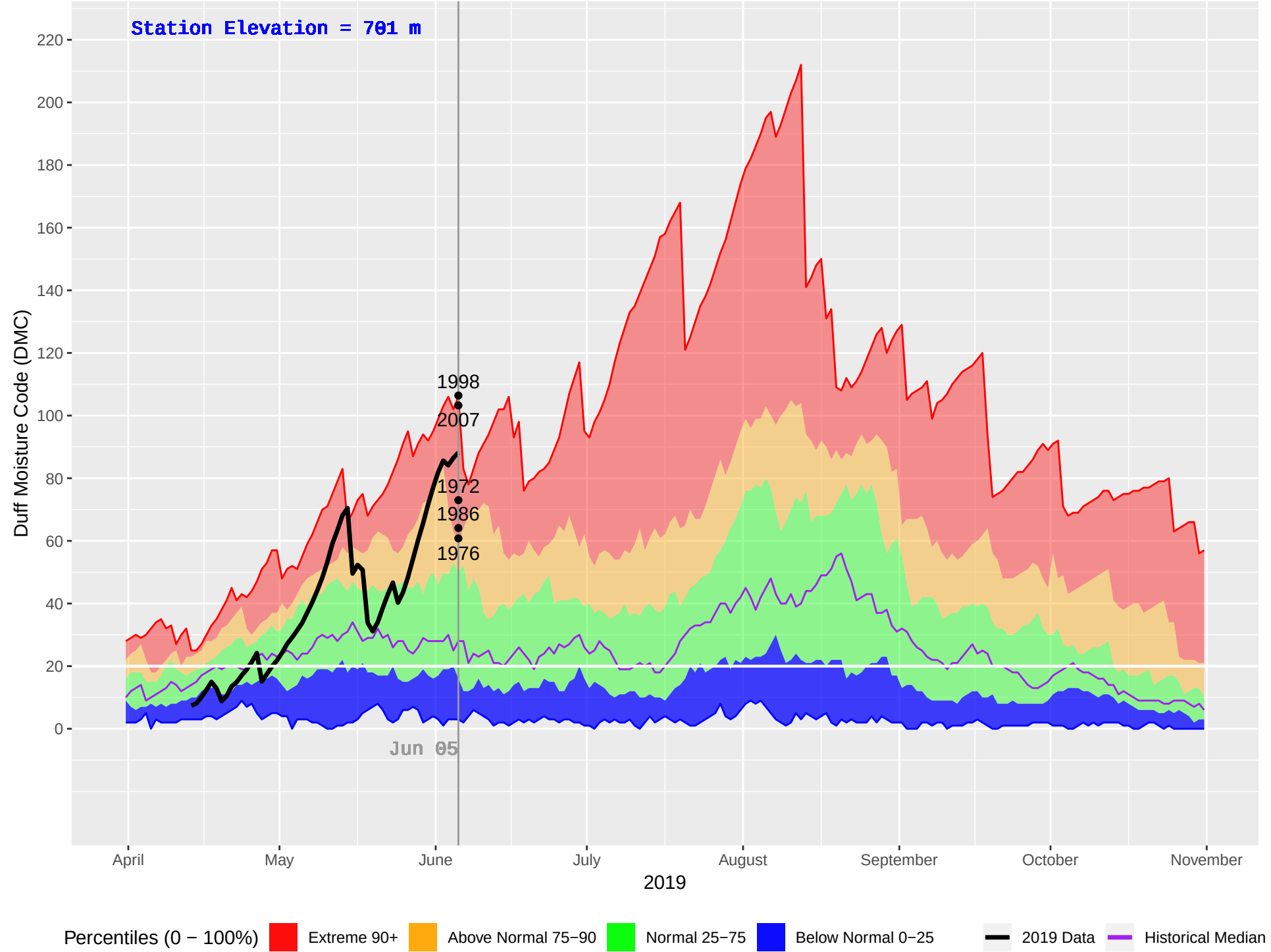
HORSEFLY (230) : Historical (1971–2018), Current (2019) Daily Duff Moisture Code (DMC)
