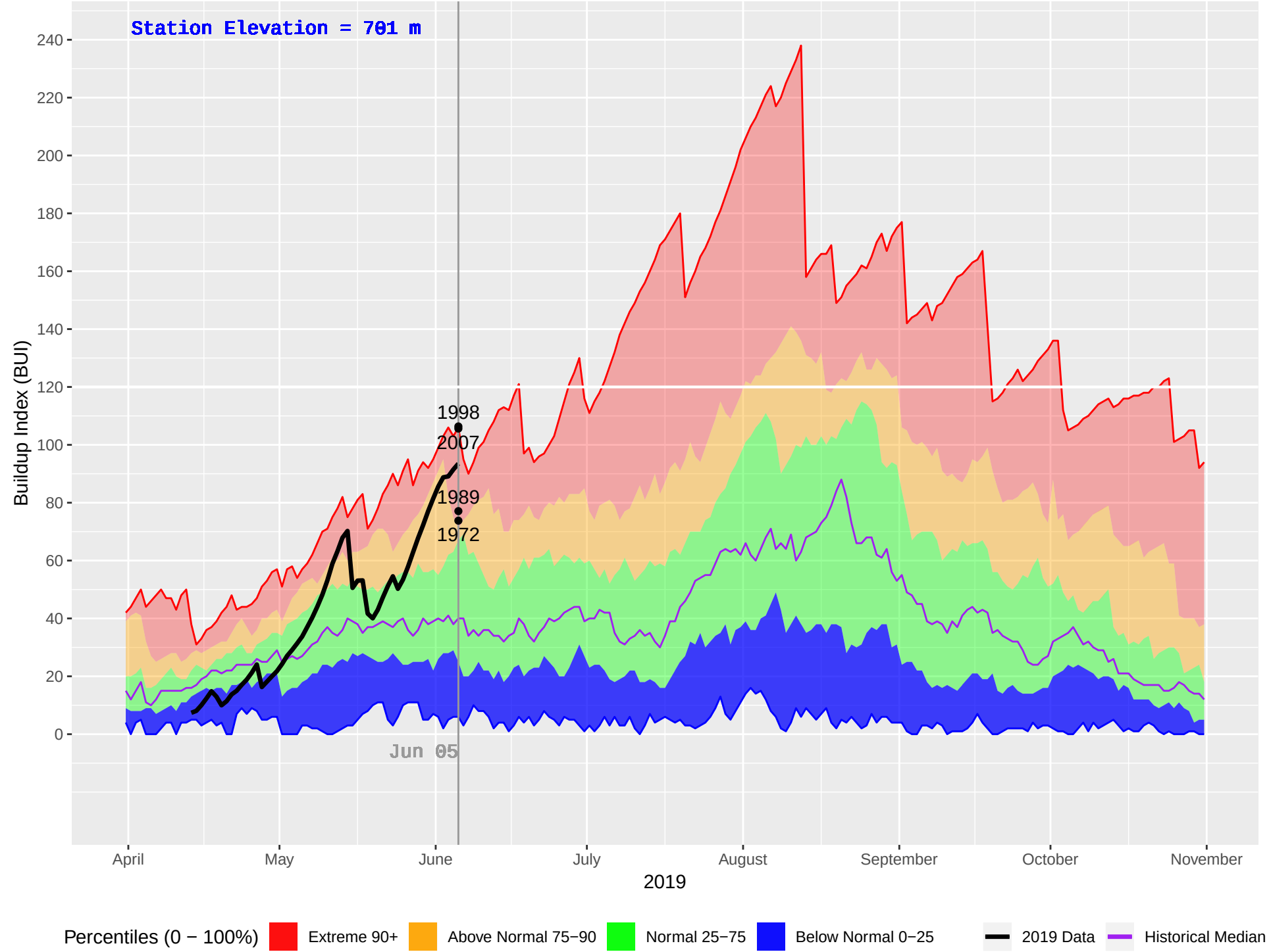
HORSEFLY (230) : Historical (1971–2018), Current (2019) Daily Buildup Index (BUI)
