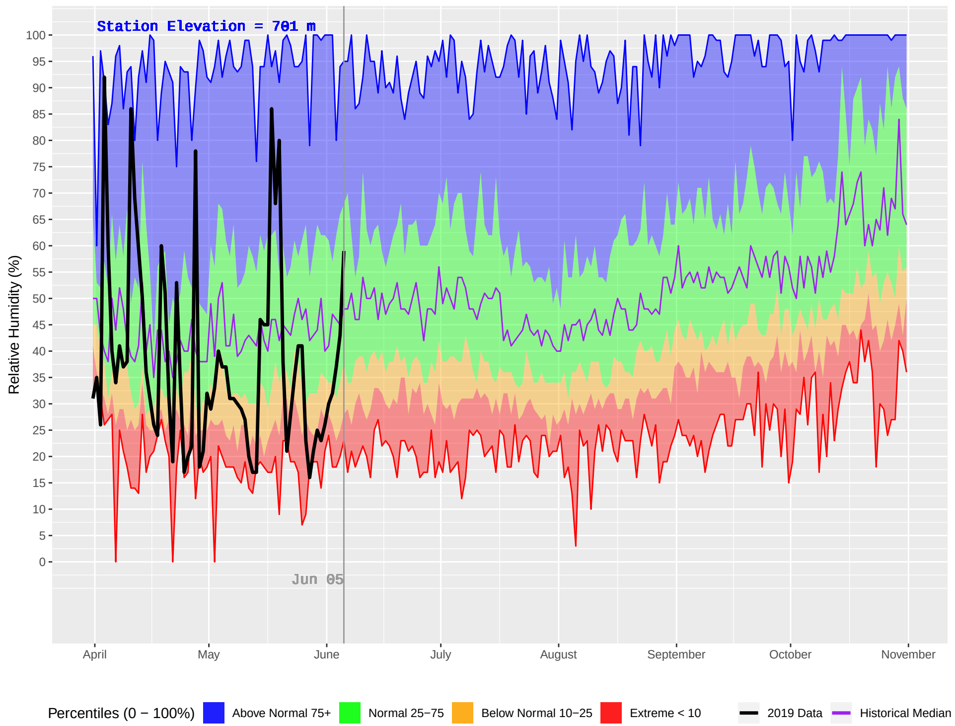
HORSEFLY (230) : Historical (1971–2018) and Current (2019) Daily Relative Humidity
